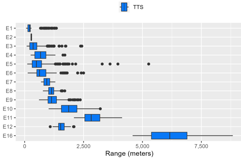
Figure E.2-38: Sirenian Ranges to Temporary Threshold Shift for Explosives
