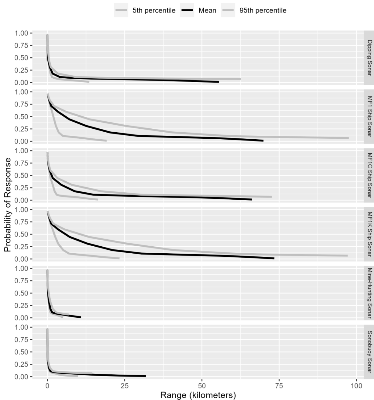
Figure E.2-18: Probability of Behavioral Response to Sonar as a Function of Range for Odontocetes
