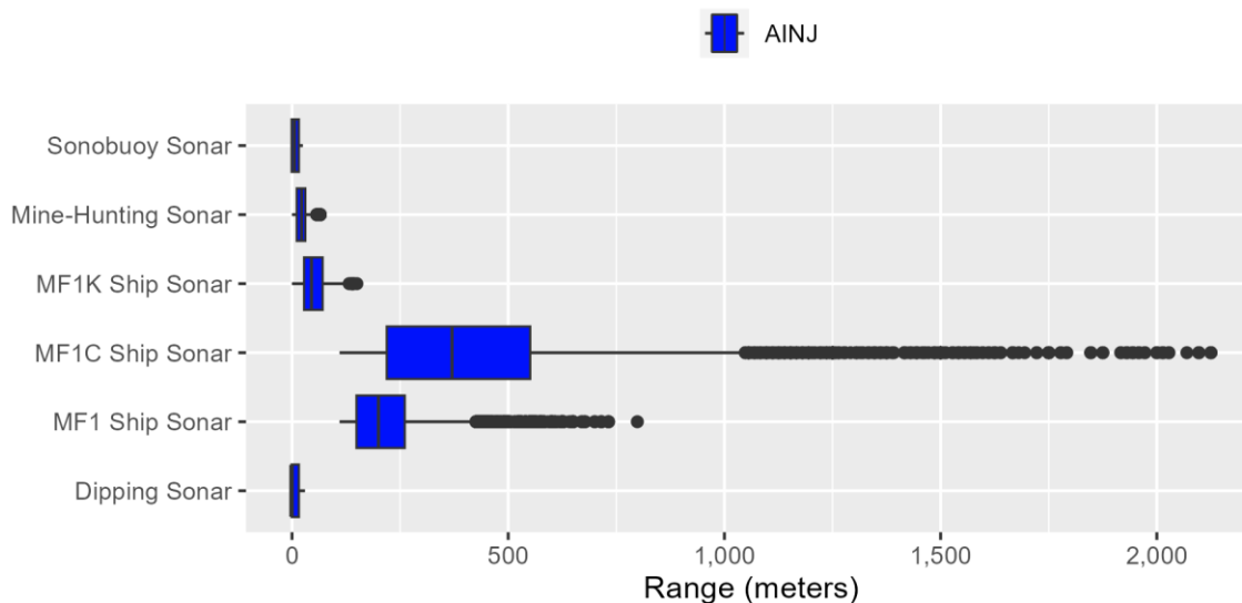
Figure E.2-13: Very High Frequency Cetacean Ranges to Auditory Injury for Sonar
