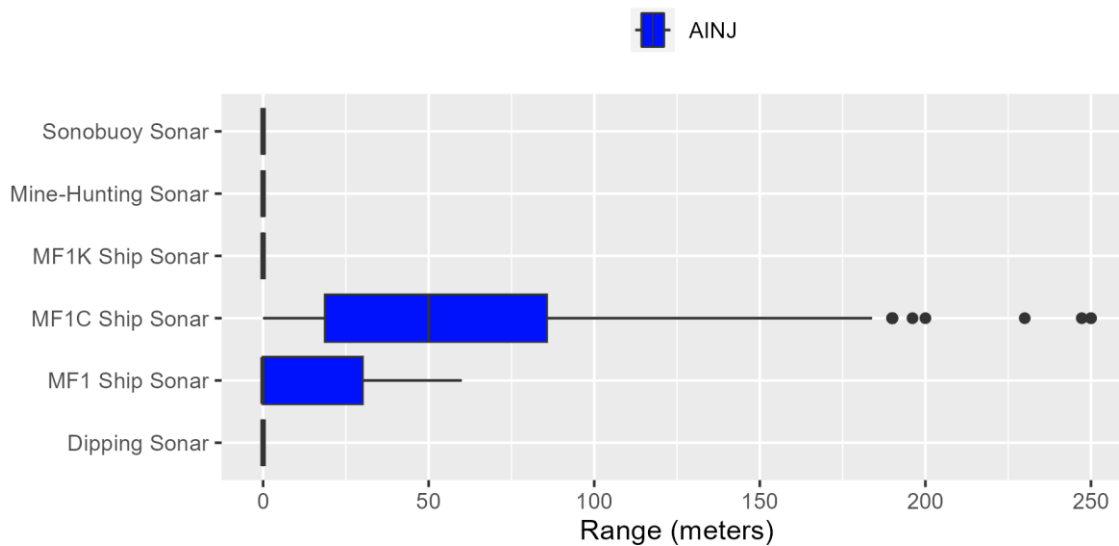
Figure E.2-17: Sirenian Ranges to Auditory Injury for Sonar
