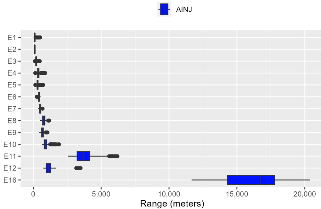
Figure E.2-24: Very Low Frequency Cetacean Ranges to Auditory Injury for Explosives
