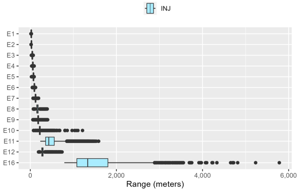
Figure E.2-40: Explosive Ranges to Injury for All Marine Mammal Hearing Groups
