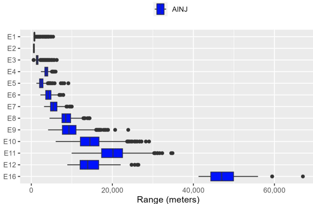
Figure E.2-33: Very High Frequency Cetacean Ranges to Auditory Injury for Explosives
