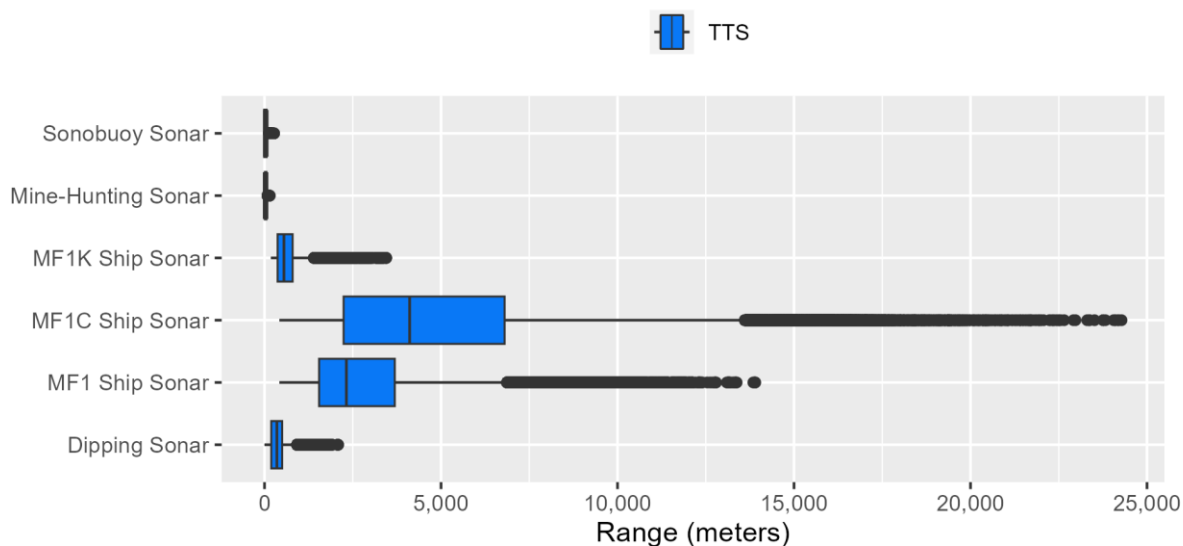
Figure E.2-14: Phocid Carnivores in Water Ranges to Temporary Threshold Shift for Sonar
