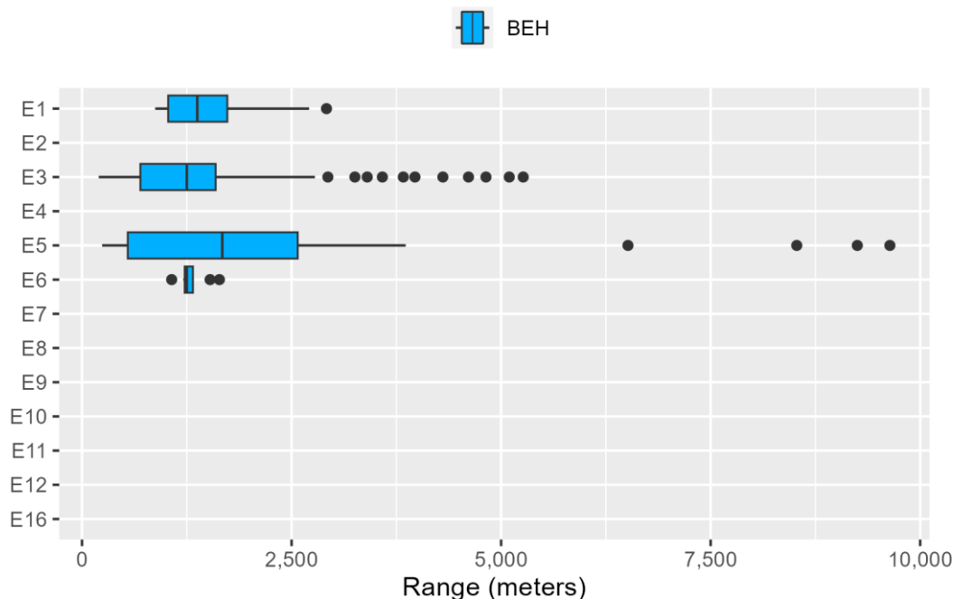
Figure E.2-37: Sirenian Ranges to Behavioral Response for Explosives
