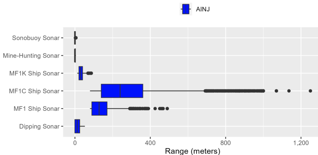
Figure E.2-9: Low Frequency Cetacean Ranges to Auditory Injury for Sonar
