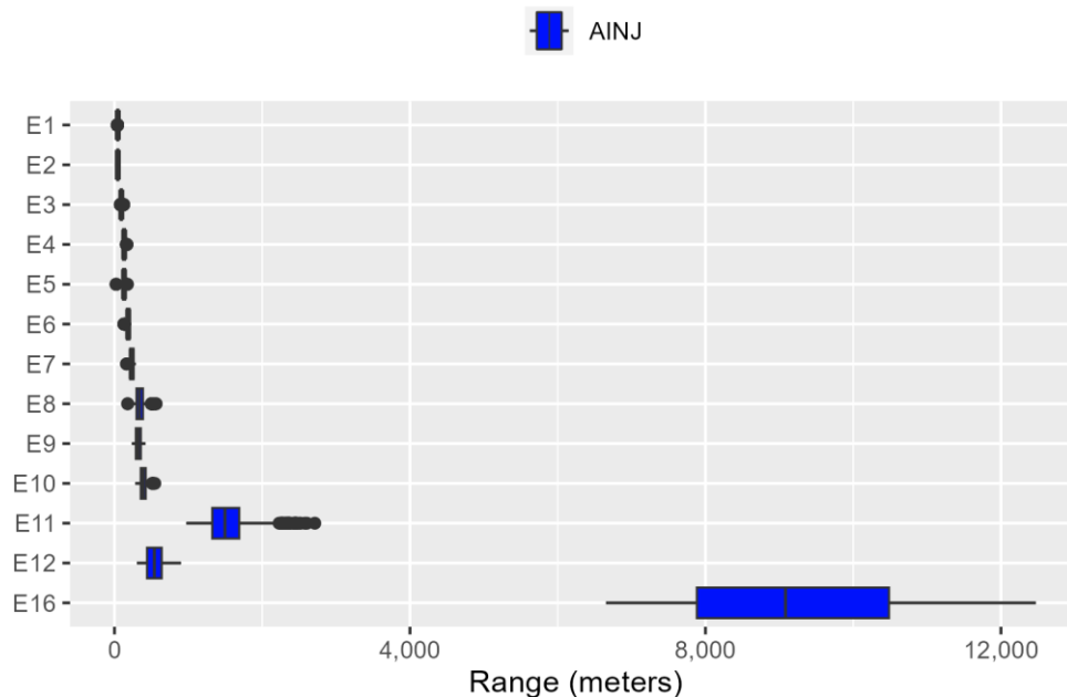
Figure E.3-4: Sea Turtle Ranges to Auditory Injury for Explosives
