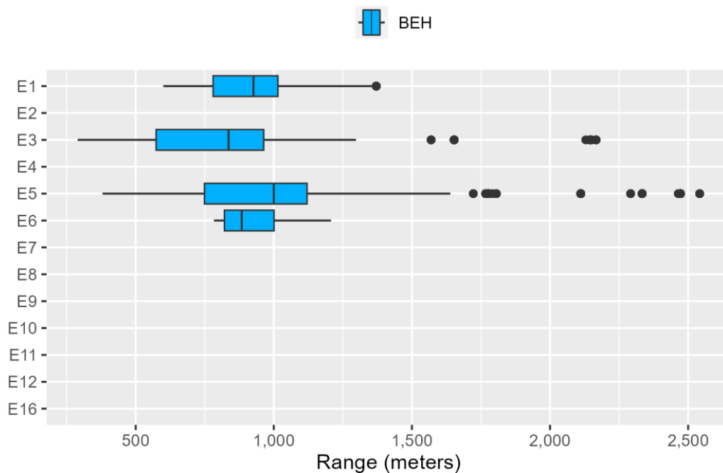
Figure E.2-28: High Frequency Cetacean Ranges to Behavioral Response for Explosives
