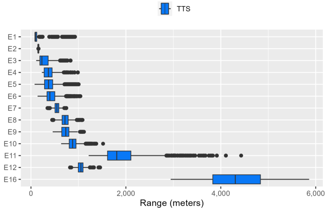
Figure E.2-29: High Frequency Cetacean Ranges to Temporary Threshold Shift for Explosives
