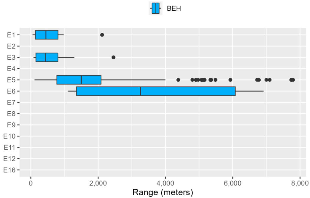
Figure E.3-2: Sea Turtle Ranges to Behavioral Response for Explosives
