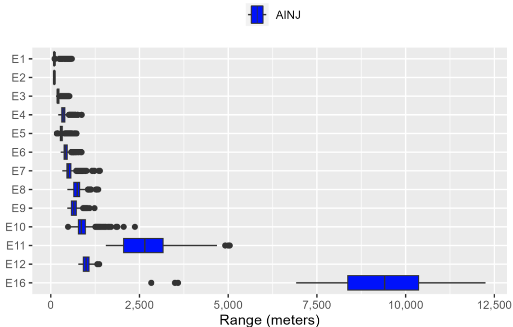
Figure E.2-27: Low Frequency Cetacean Ranges to Auditory Injury for Explosives
