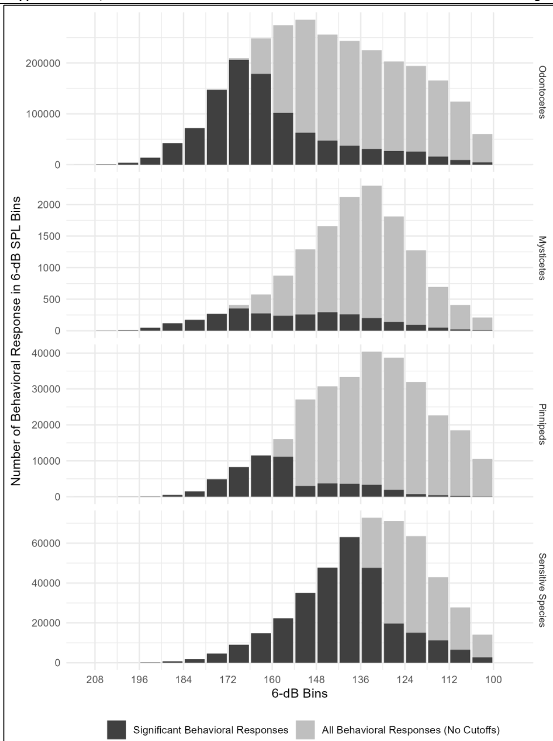
Figure E.2-4: Total predicted Instances of Marine Mammal Behavioral Responses in the Study Area by Received Level
