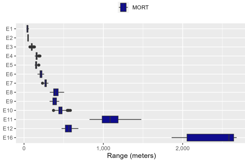
Figure E.4-5: Fishes with a Swim Bladder Ranges to Mortality for Explosives
