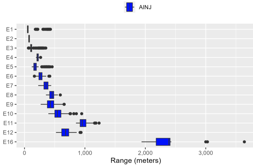
Figure E.2-39: Sirenian Ranges to Auditory Injury for Explosives
