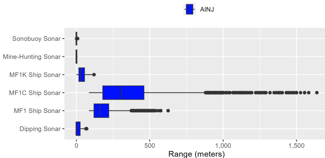
Figure E.2-15: Phocid Carnivores in Water Ranges to Auditory Injury for Sonar
