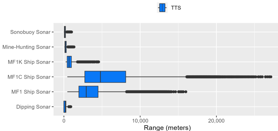
Figure E.2-12: Very High Frequency Cetacean Ranges to Temporary Threshold Shift for Sonar
