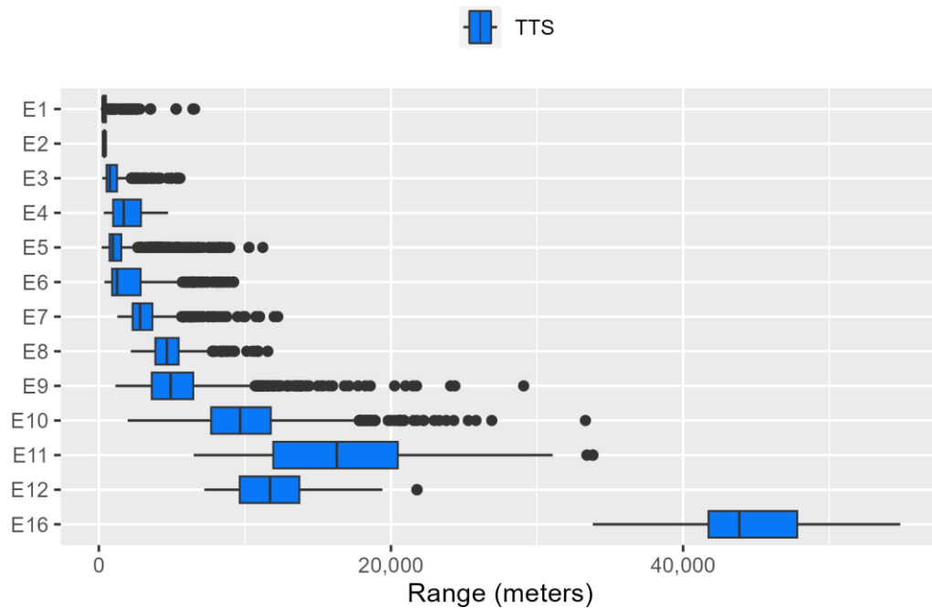
Figure E.2-26: Low Frequency Cetacean Ranges to Temporary Threshold Shift for Explosives
