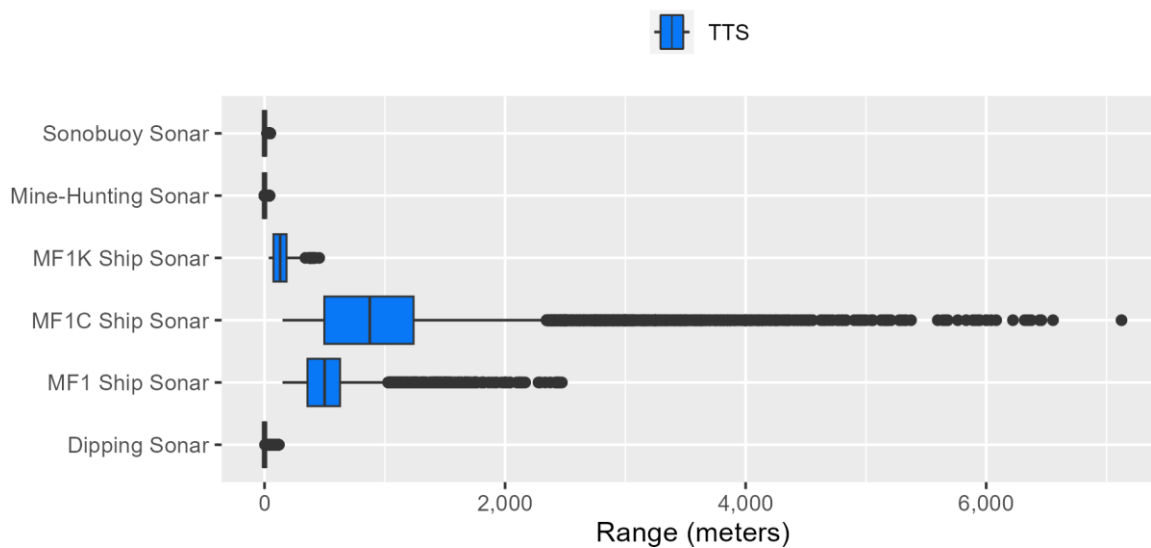
Figure E.2-16: Sirenian Ranges to Temporary Threshold Shift for Sonar
