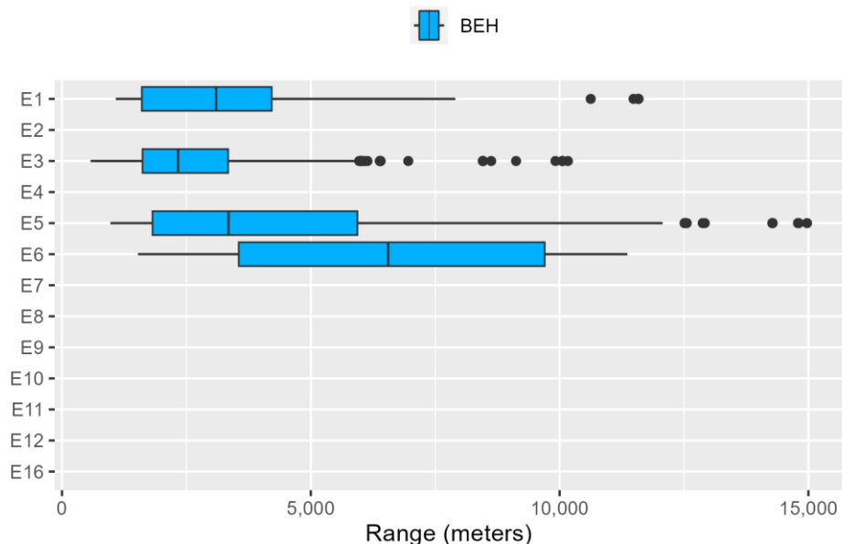
Figure E.2-34: Phocid Carnivores in Water Ranges to Behavioral Response for Explosives
