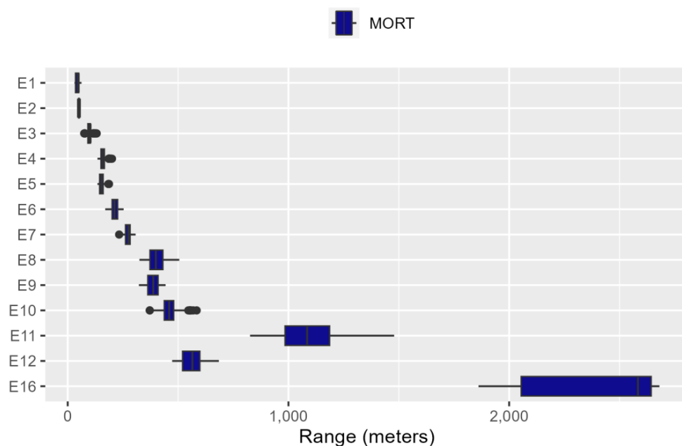
Figure E.4-2: Fishes without a Swim Bladder Ranges to Mortality for Explosives
