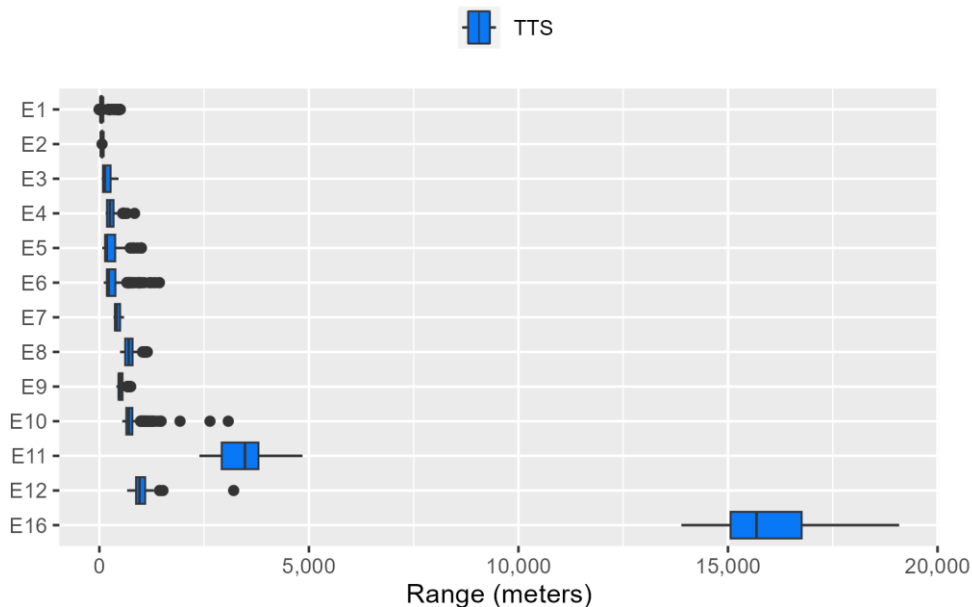
Figure E.4-3: Fishes with a Swim Bladder Ranges to Temporary Threshold Shift for Explosives
