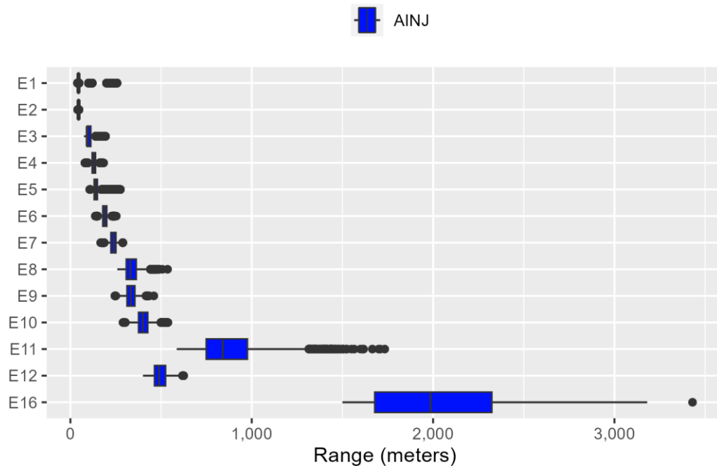
Figure E.2-30: High Frequency Cetacean Ranges to Auditory Injury for Explosives
