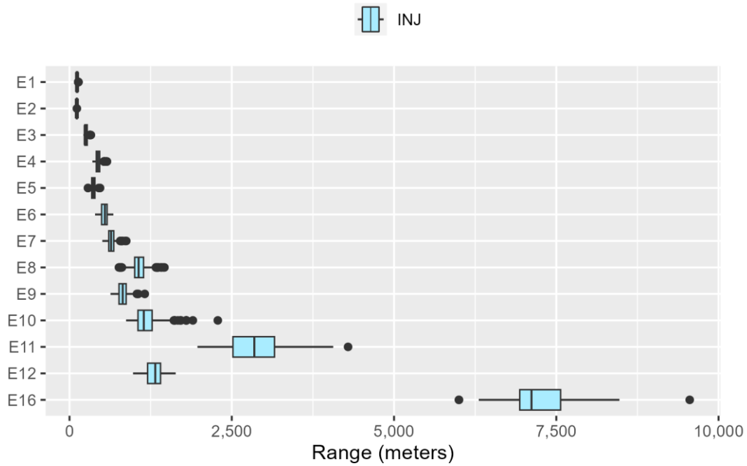
Figure E.4-4: Fishes with a Swim Bladder Ranges to Injury for Explosives
