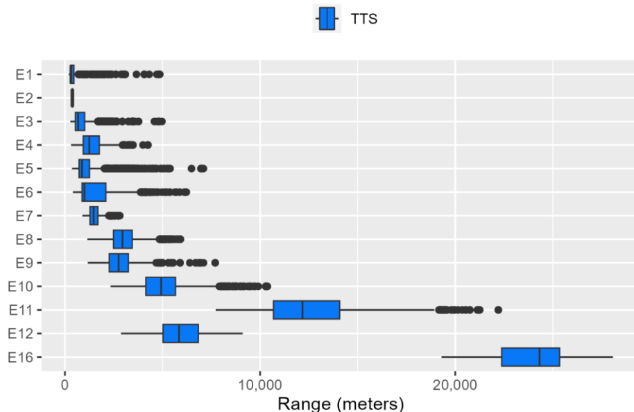
Figure E.2-35: Phocid Carnivores in Water Ranges to Temporary Threshold Shift for Explosives
