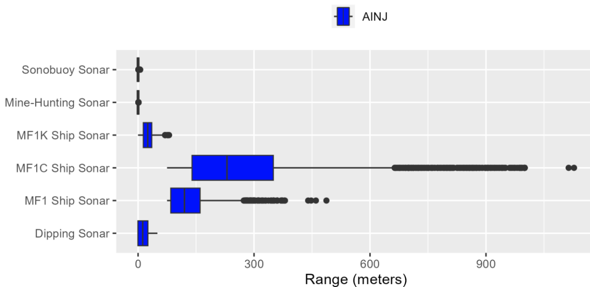
Figure E.2-7: Very Low Frequency Cetacean Ranges to Auditory Injury for Sonar
