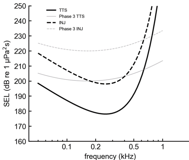
Figure E.3-1: Sea Turtle Exposure Function for Non-Impulsive TTS and AINJ
