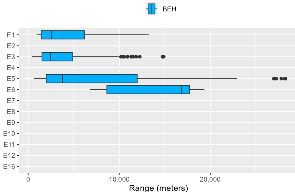
Figure E.2-22: Very Low Frequency Cetacean Ranges to Behavioral Response for Explosives
