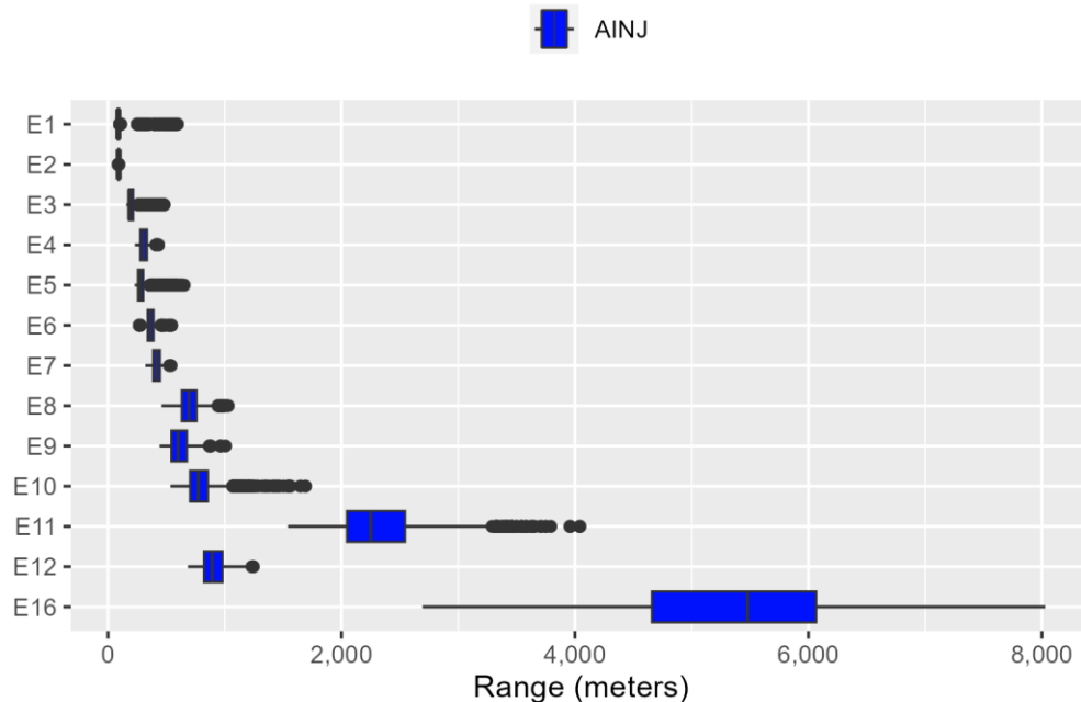
Figure E.2-36: Phocid Carnivores in Water Ranges to Auditory Injury for Explosives
