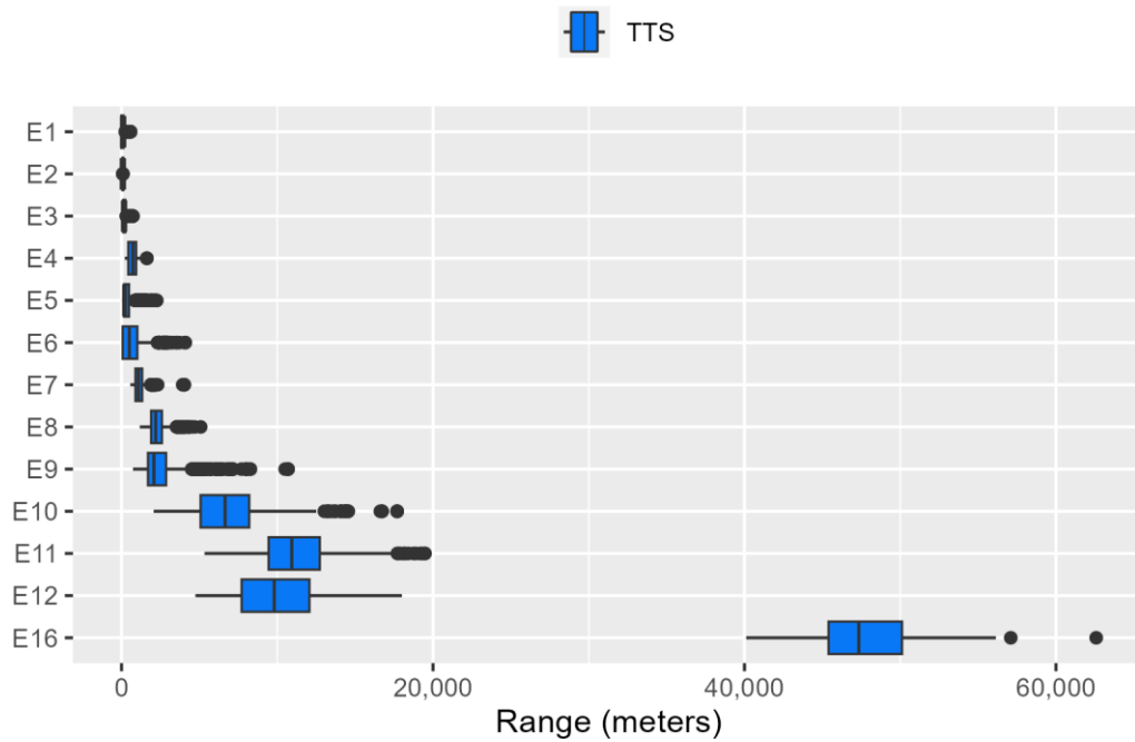
Figure E.3-3: Sea Turtle Ranges to Temporary Threshold Shift for Explosives
