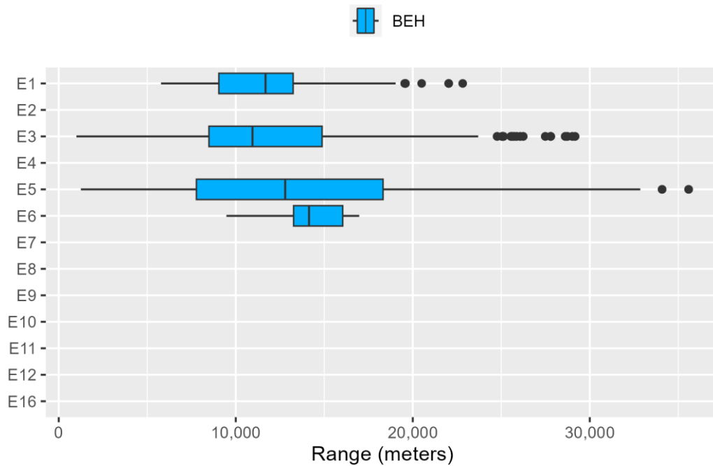
Figure E.2-31: Very High Frequency Cetacean Ranges to Behavioral Response for Explosives
