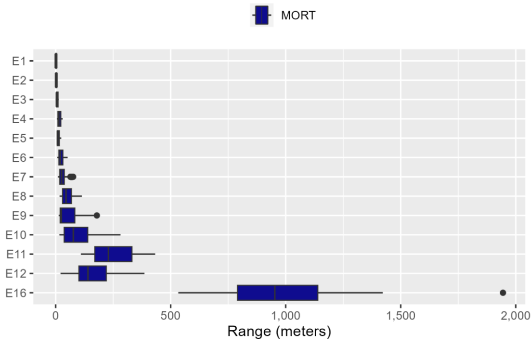
Figure E.3-6: Explosive Ranges to Mortality for Sea Turtles
