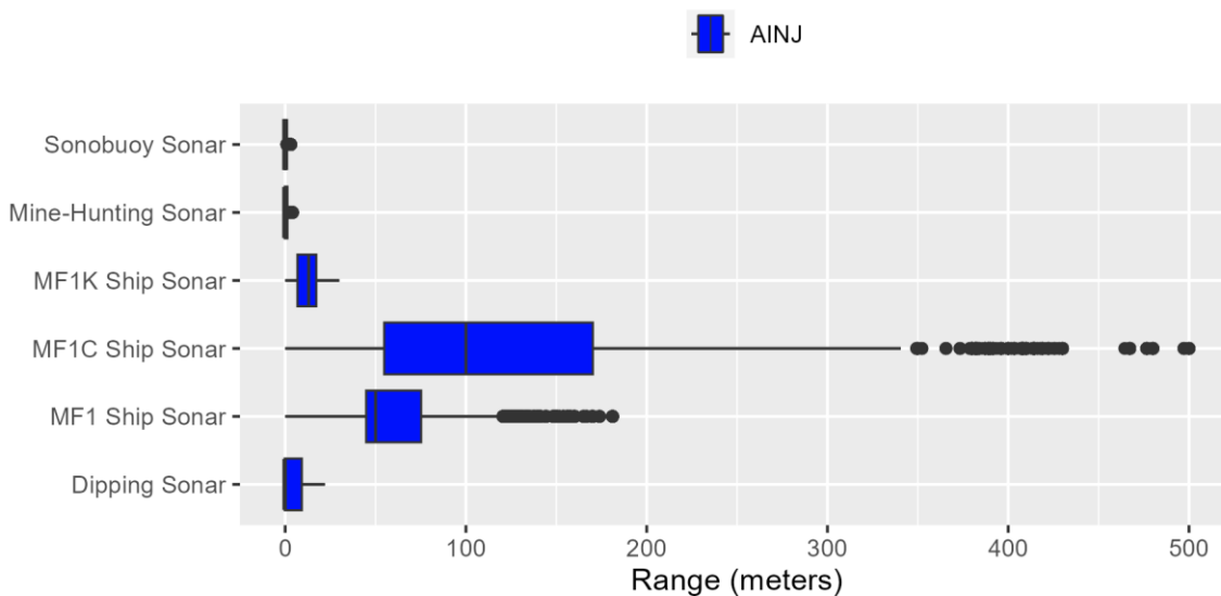
Figure E.2-11: High Frequency Cetacean Ranges to Auditory Injury for Sonar
