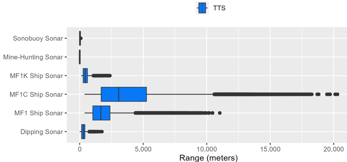
Figure E.2-6: Very Low Frequency Cetacean Ranges to Temporary Threshold Shift for Sonar
