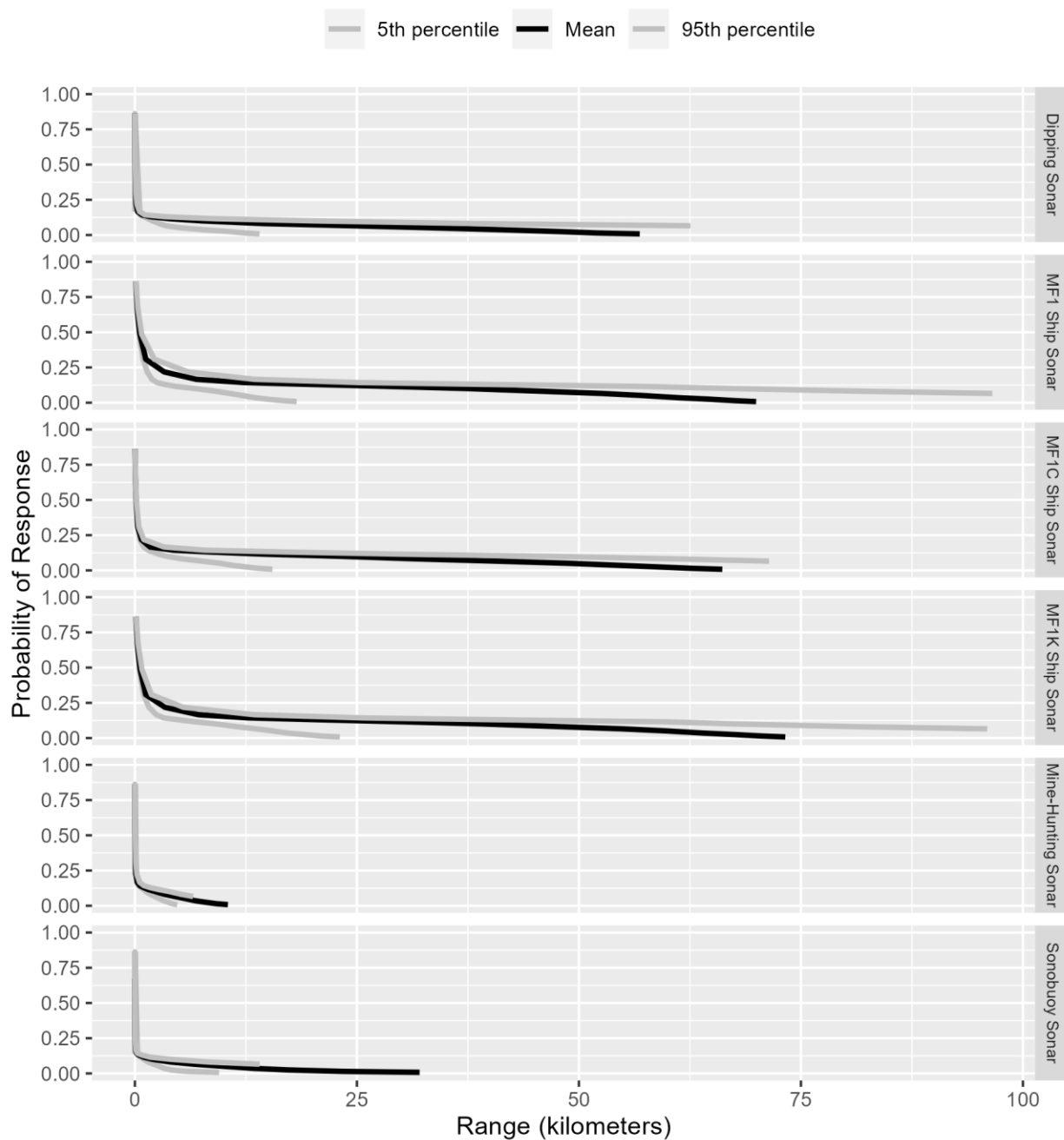
Figure E.2-19: Probability of Behavioral Response to Sonar as a Function of Range for Mysticetes
