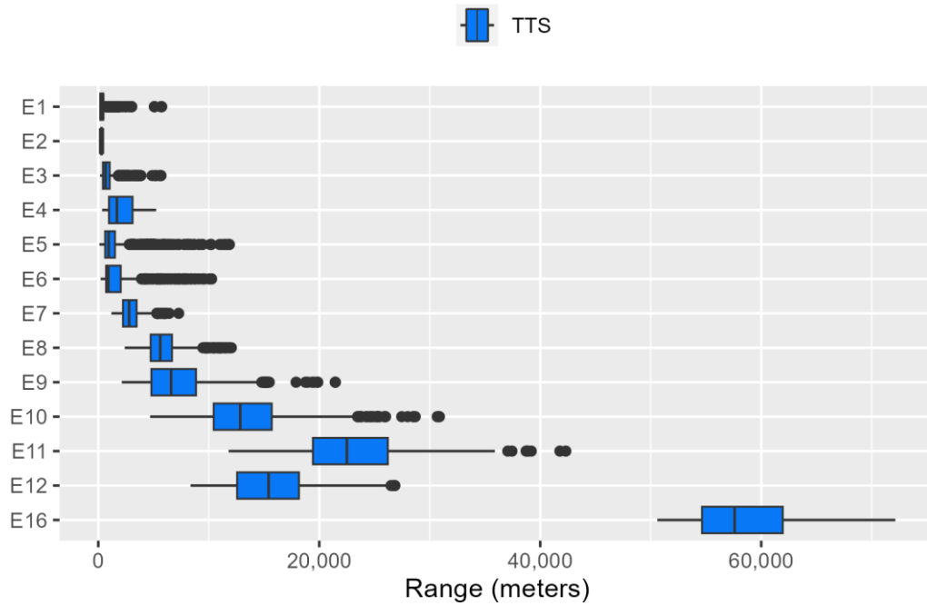
Figure E.2-23: Very Low Frequency Cetacean Ranges to Temporary Threshold Shift for Explosives
