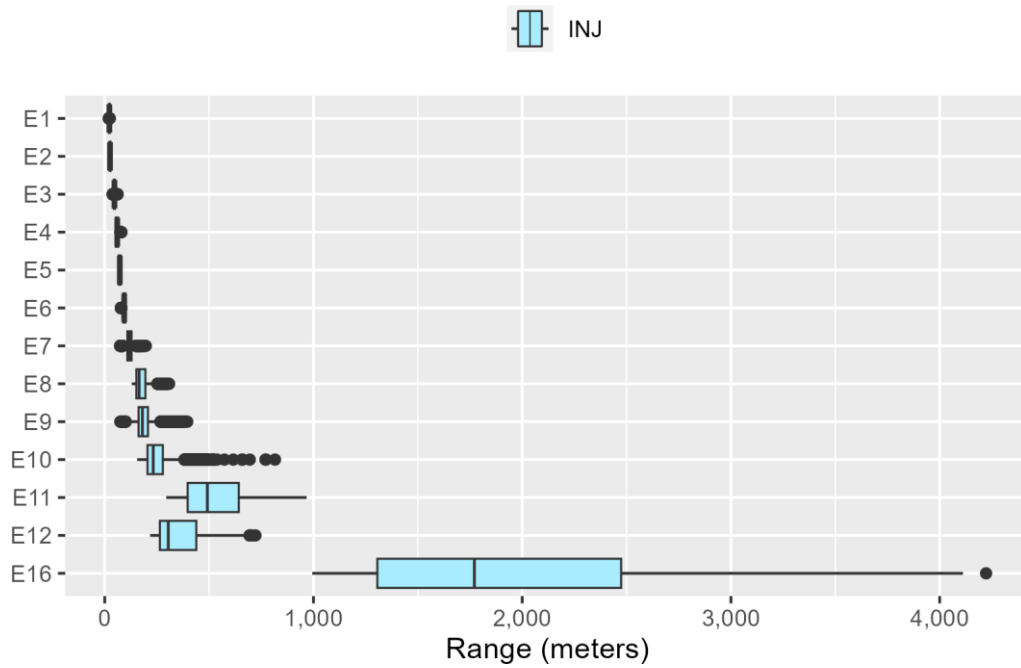
Figure E.3-5: Explosive Ranges to Injury for Sea Turtles
