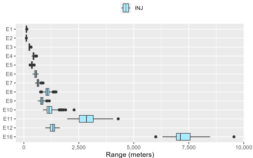
Figure E.4-1: Fishes without a Swim Bladder Ranges to Injury for Explosives
