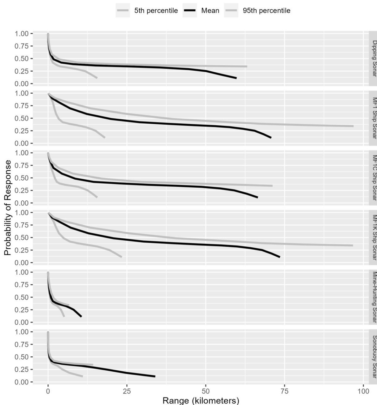
Figure E.2-21: Probability of Behavioral Response to Sonar as a Function of Range for Pinnipeds
