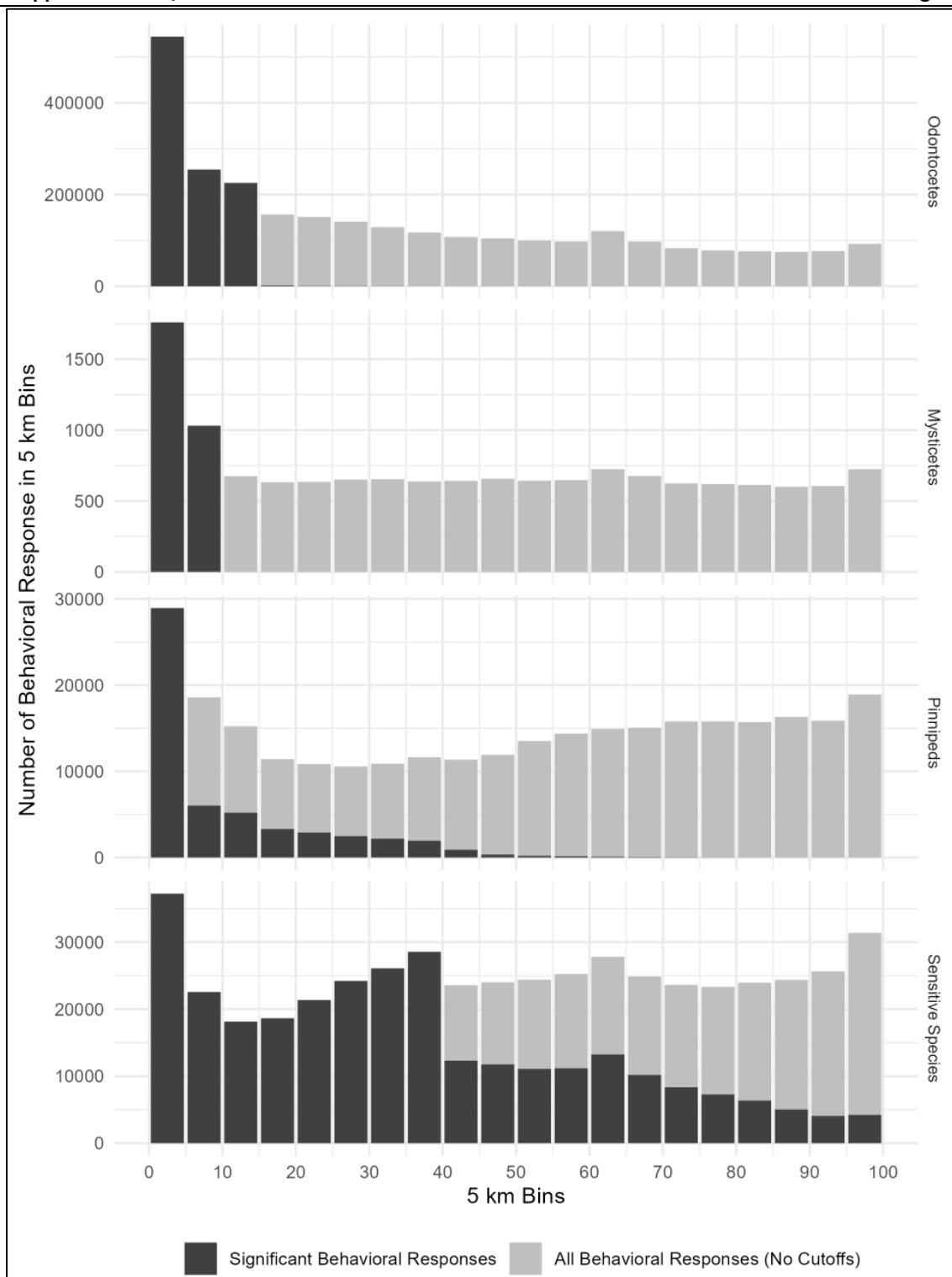
Figure E.2-5: Total Predicted Instances of Marine Mammal Behavioral Responses in the Study Area by Distance
