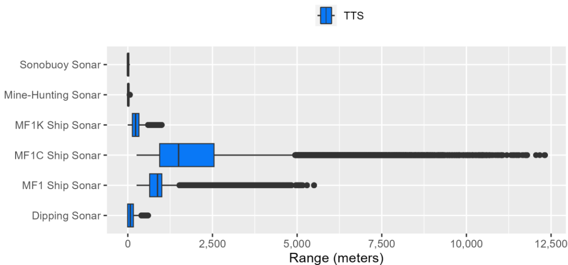
Figure E.2-10: High Frequency Cetacean Ranges to Temporary Threshold Shift for Sonar
