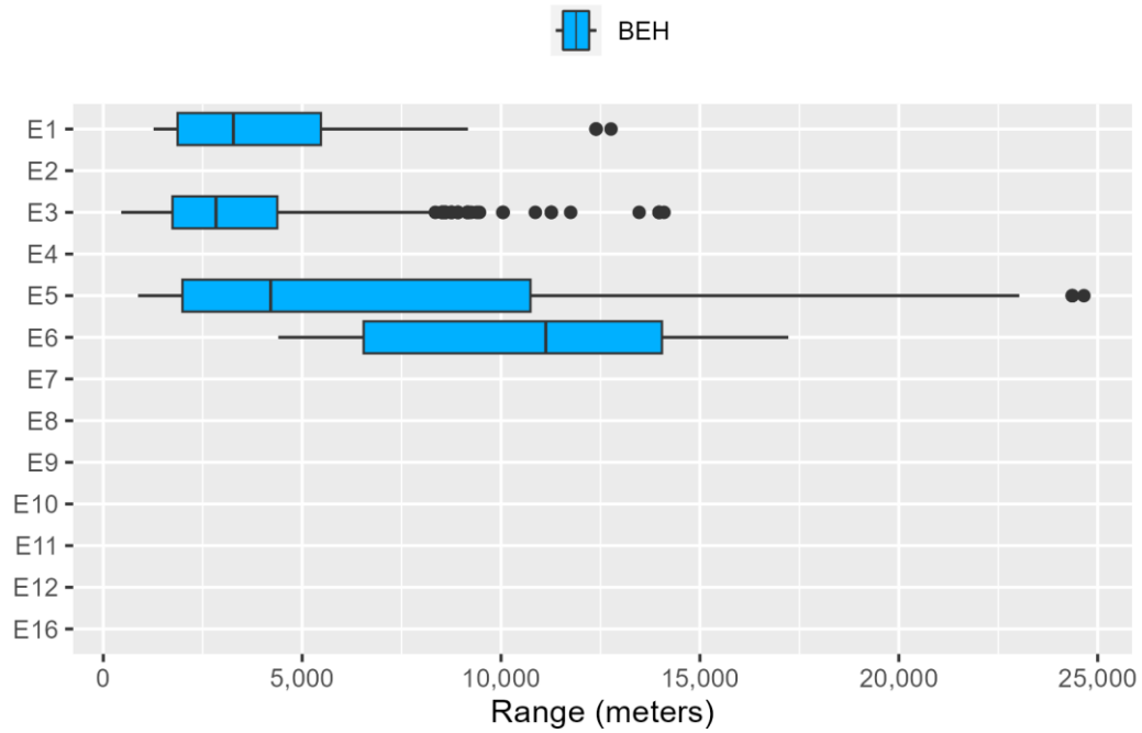
Figure E.2-25: Low Frequency Cetacean Ranges to Behavioral Response for Explosives
