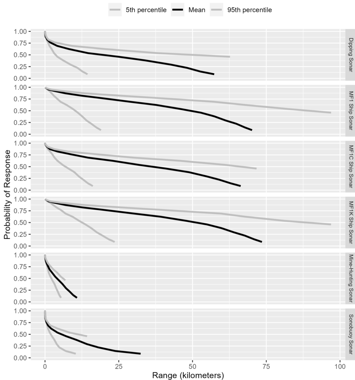
Figure E.2-20: Probability of Behavioral Response to Sonar as a Function of Range for Sensitive Species
