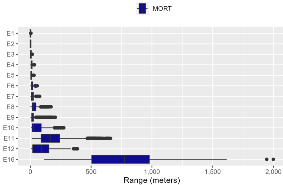
Figure E.2-41: Explosive Ranges to Mortality for All Marine Mammal Hearing Groups
