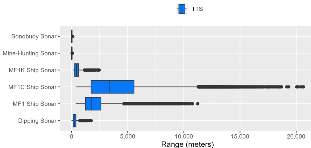
Figure E.2-8: Low Frequency Cetacean Ranges to Temporary Threshold Shift for Sonar
