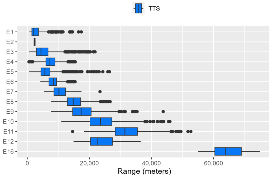
Figure E.2-32: Very High Frequency Cetacean Ranges to Temporary Threshold Shift for Explosives
